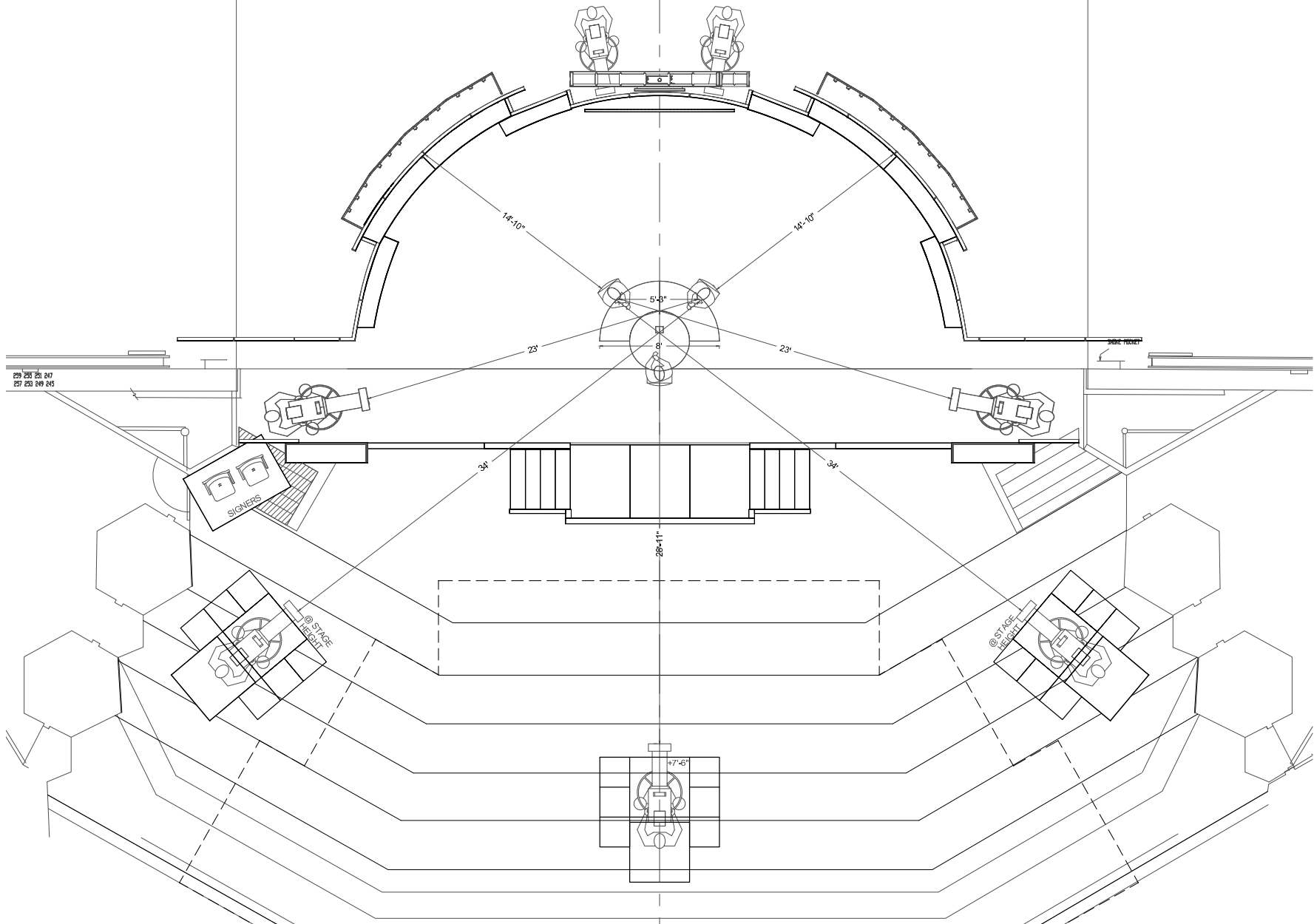
PLAN VIEW SCALE: NTS
